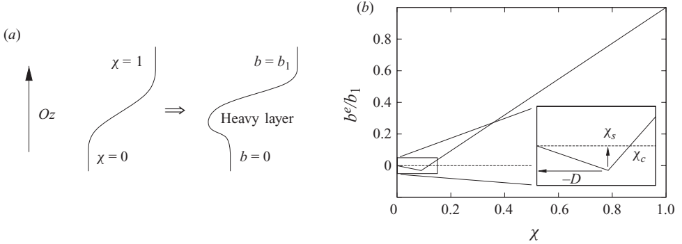
FIGURE 1. Vertical structure of the cloud top (a) in terms of the mixture fraction \chi and the buoyancy b . Buoyancy mixing function b^e(\chi) from (2.2) for reference case A11 in table 1; inset shows the associated parameters (b).
