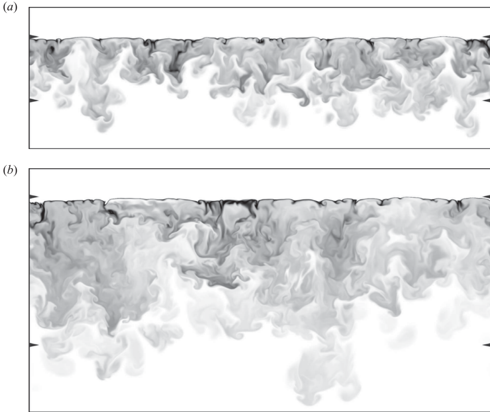
FIGURE 2. Evolution inside a vertical plane of the negative buoyancy field, with grey scale varying between black for b=b_s (minimum) and white for zero: (a) t_1(B_s/\delta_{\chi,0}^2)^{1/3}=7.96 ; (b) t_2(B_s/\delta_{\chi,0}^2)^{1/3}=15.4 . Upper triangular side marks indicate the position of the inversion base at z=z_i , and lower ones correspond to z=z_i-z^* .
